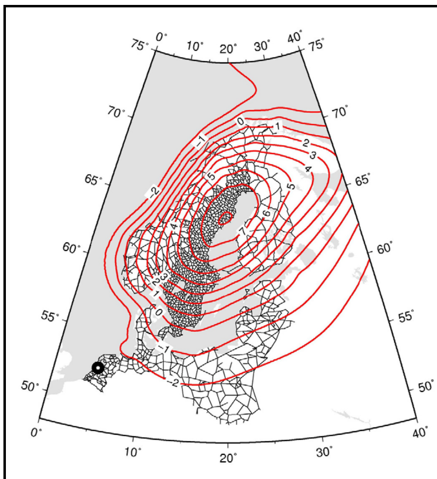
Figure 1: The network of the Baltic Levelling Ring and Fennoscandian postglacial land uplift relative to mean sea level (Mäkinen J. & al. 2006)
