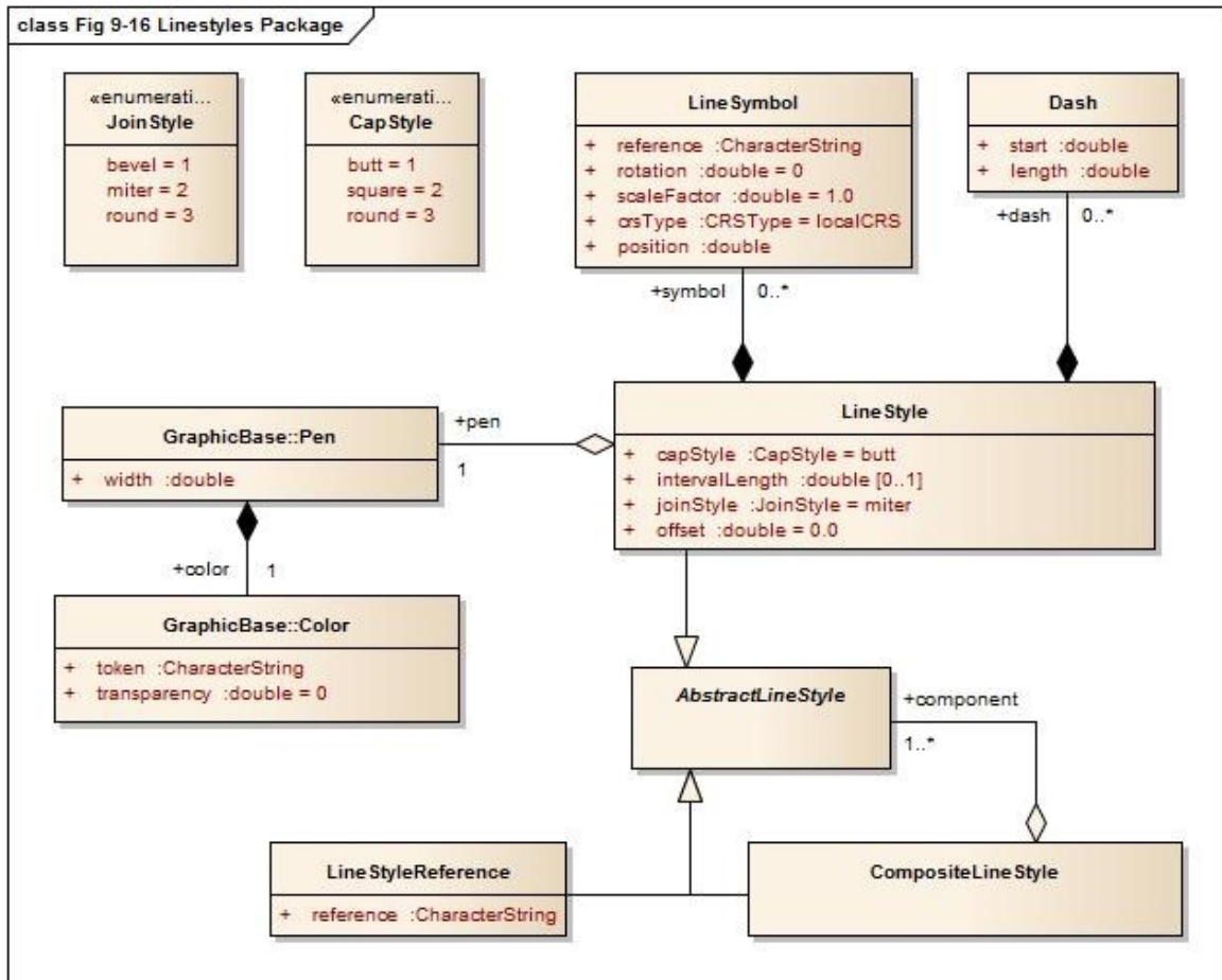
Figure 9-16 — Line Styles Package
