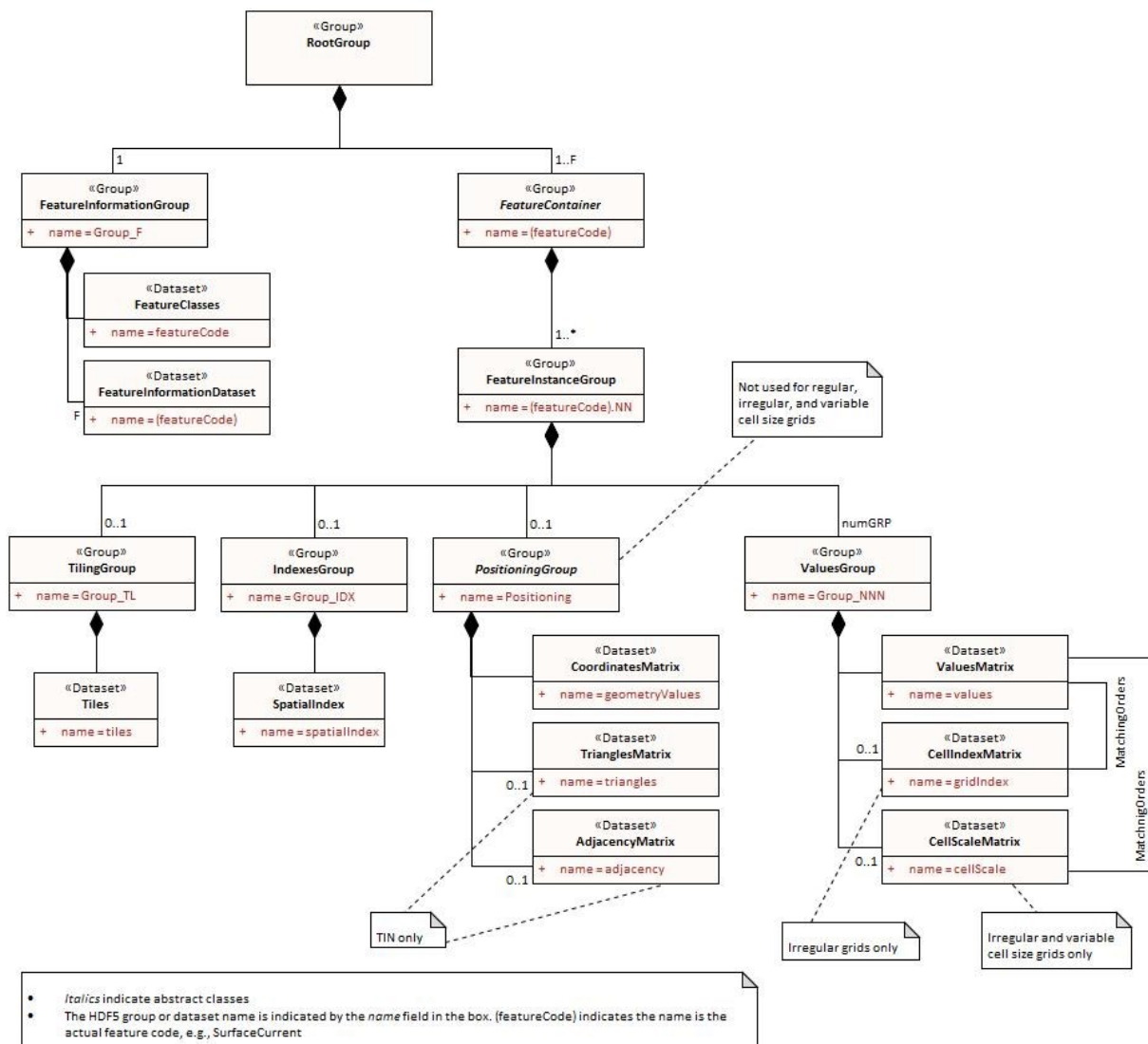
Figure 10c-12 - Conceptual model of content
