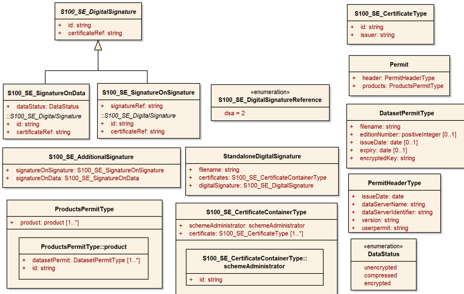
Figure 15-8 – Data protection – class details
