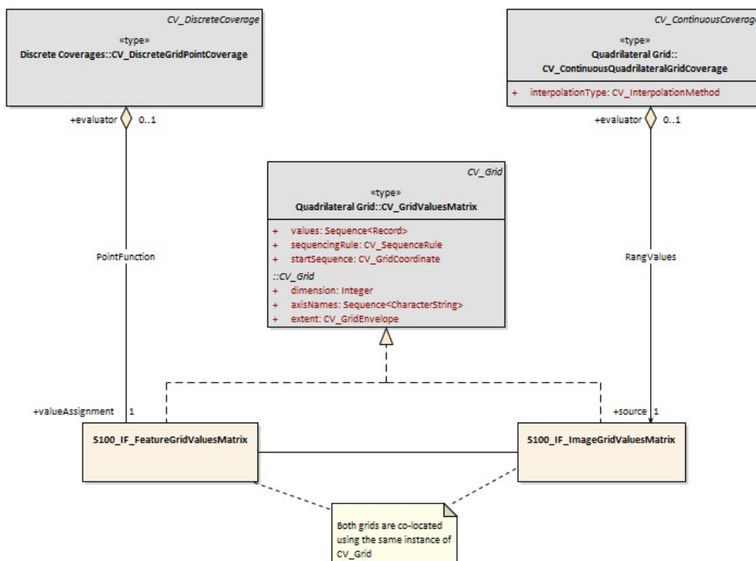
Figure 8-E-2 – Assigning feature codes to pixels in an image.
