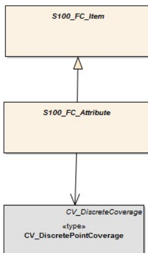
Figure 8-29 – Feature oriented discrete coverage
