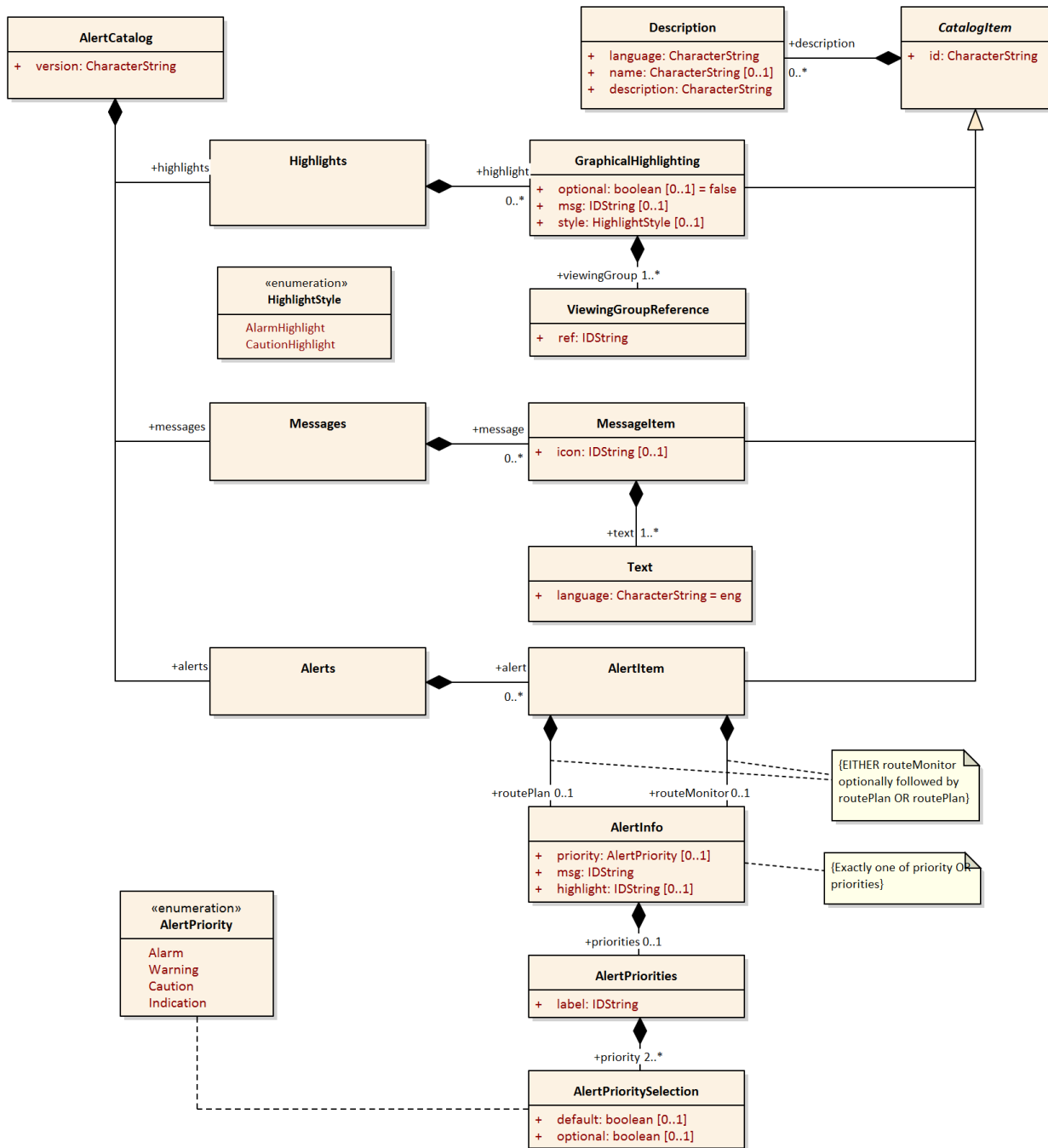
Figure 9-21 — Alert Catalogue
