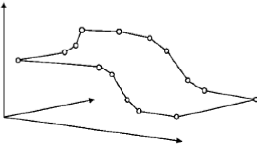
Figure 7-A-3 – 2.5D Example
