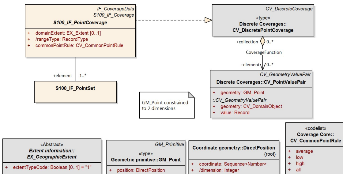
Figure 8-22 – S100_IF_PointCoverage
