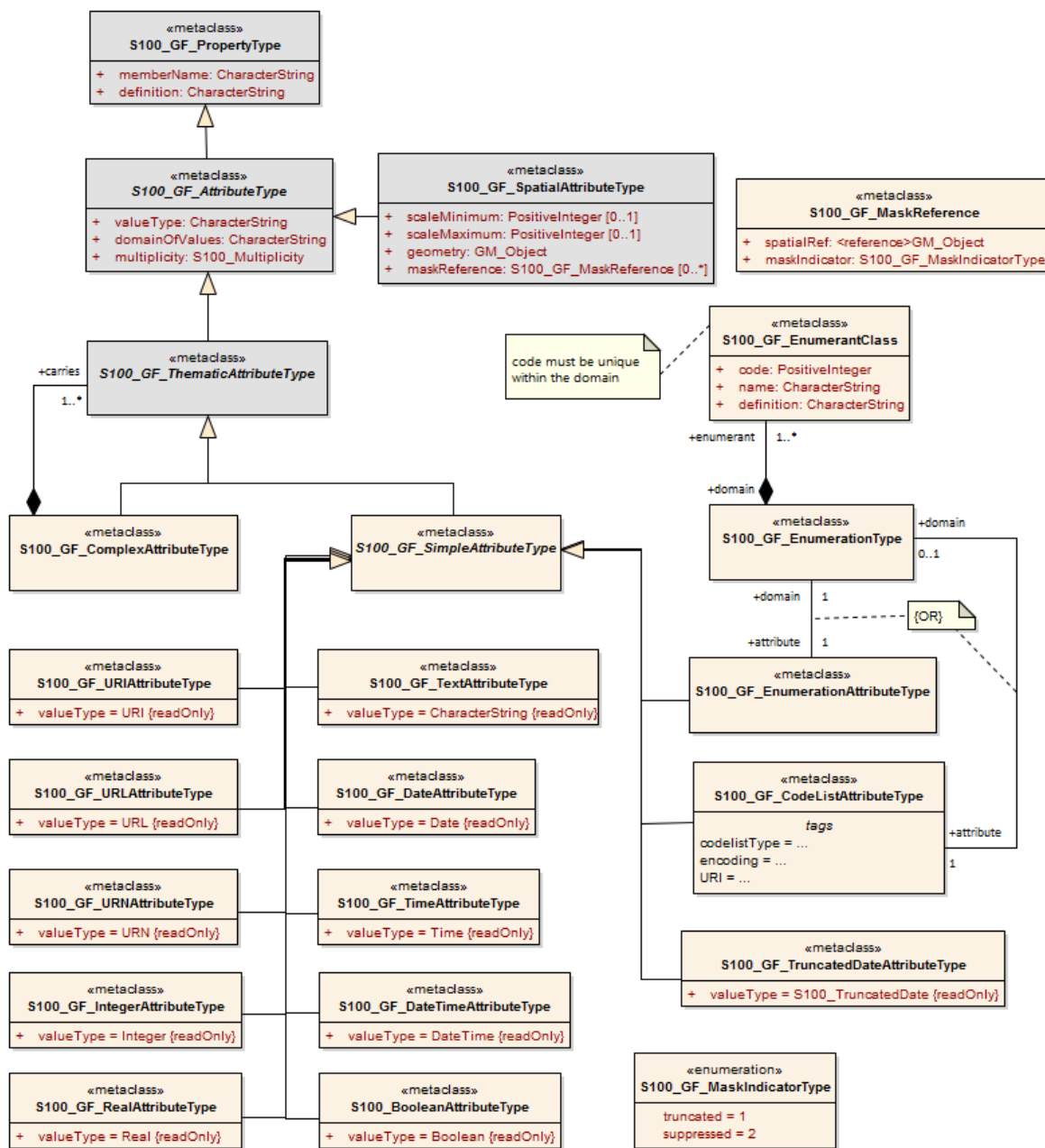
Figure 3-2 — Attributes
