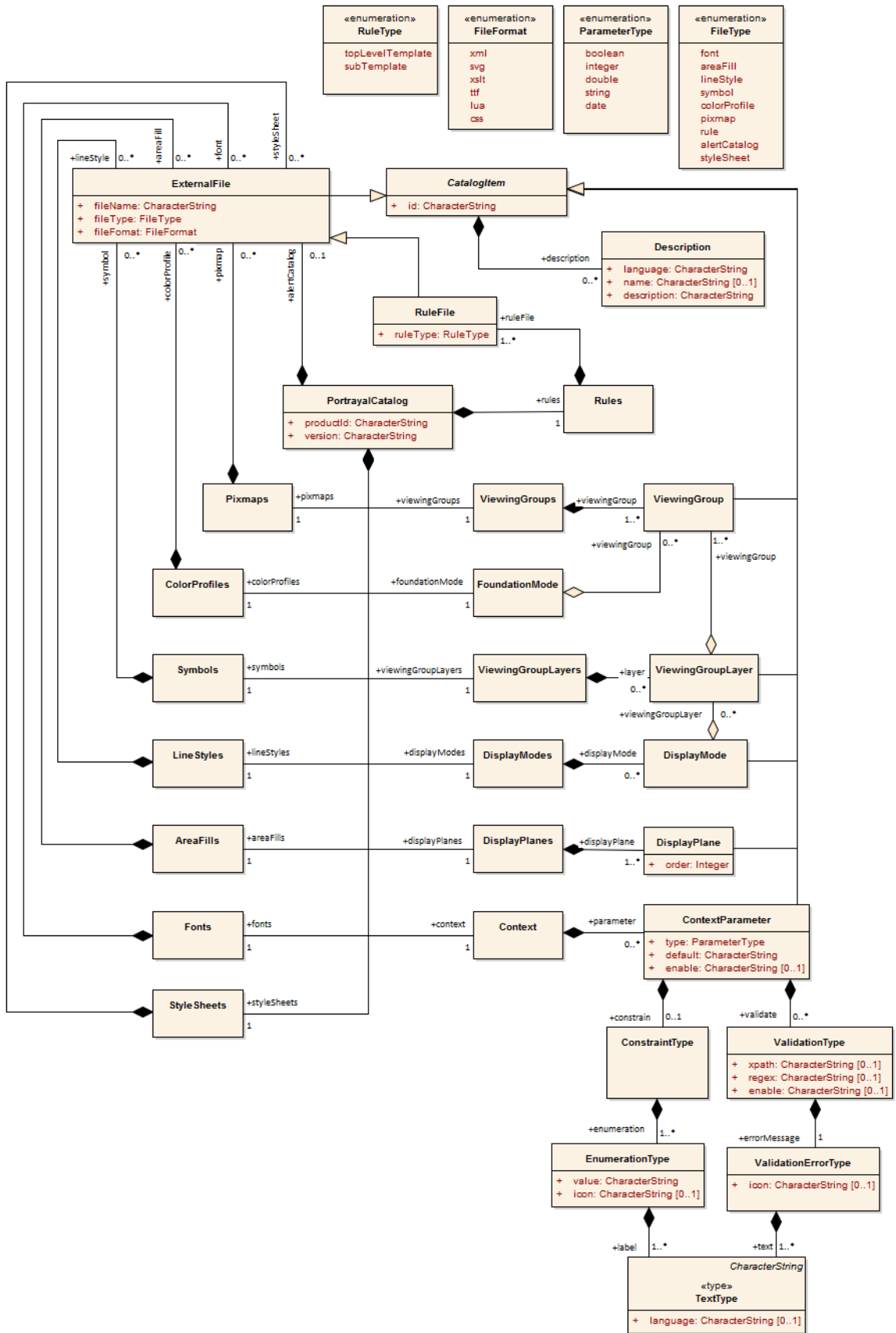
Figure 9-20 — Catalogue
