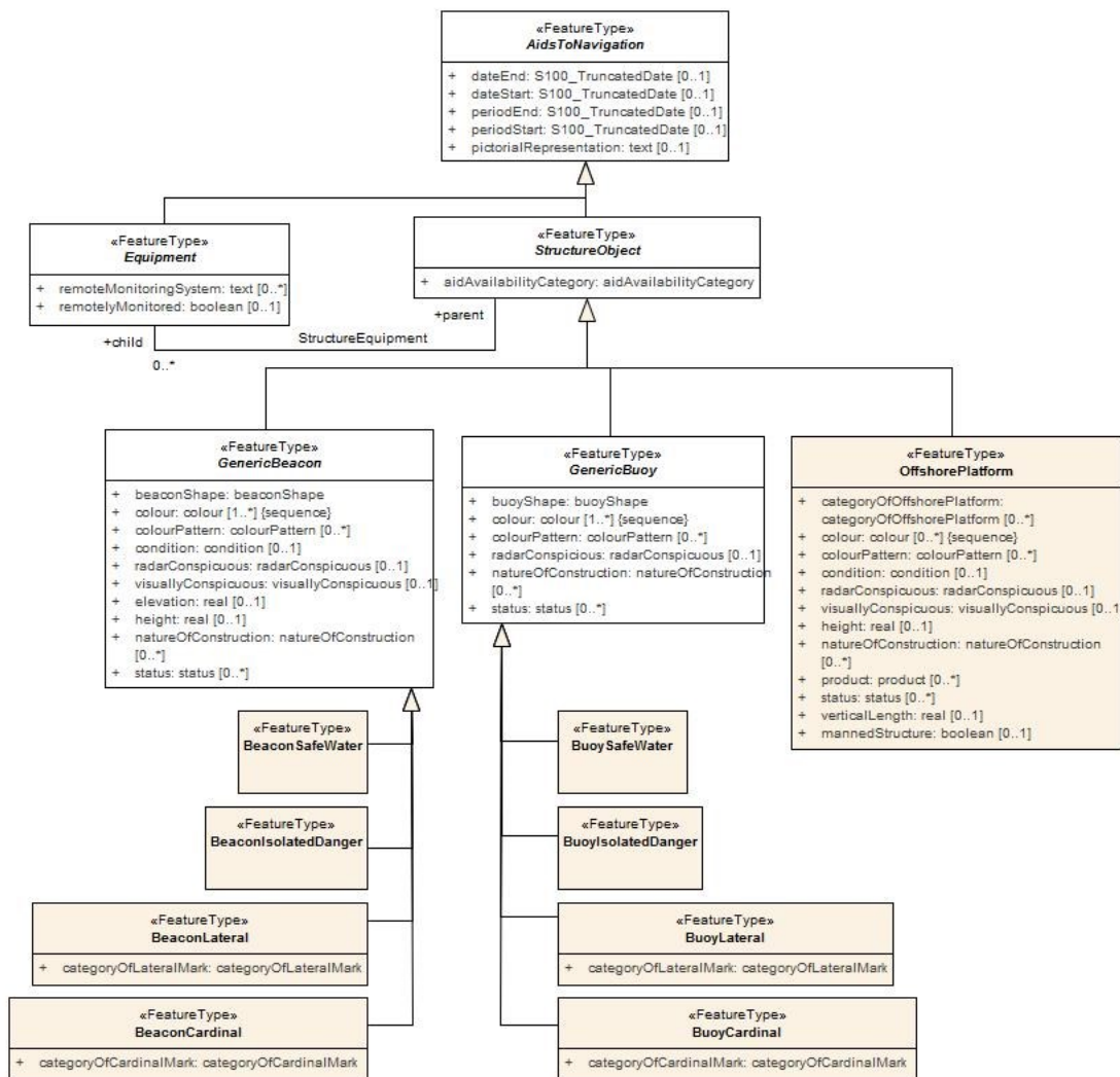
Figure 5-1 – Inheritance Example
