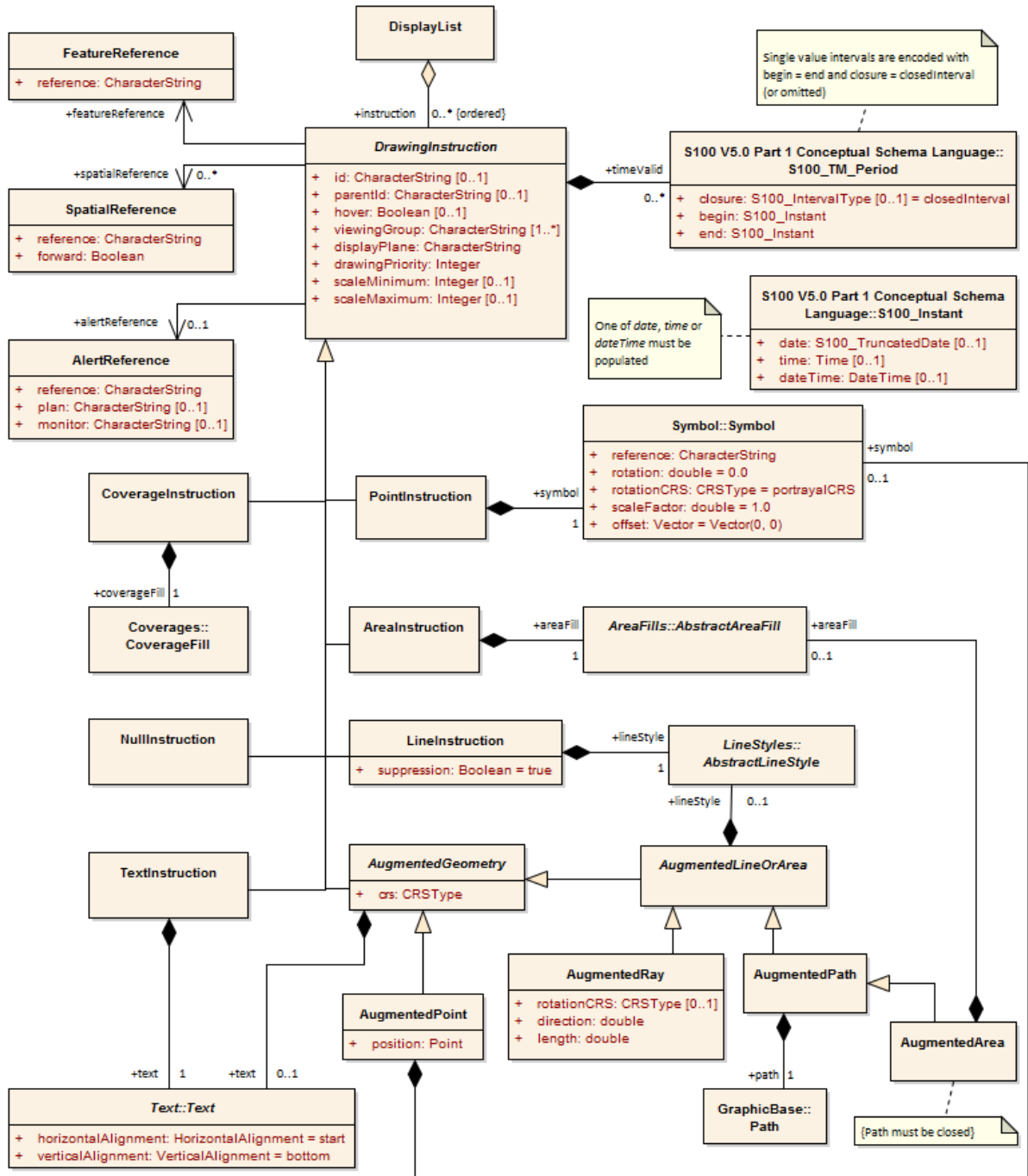
Figure 9-10 — Drawing Instructions
