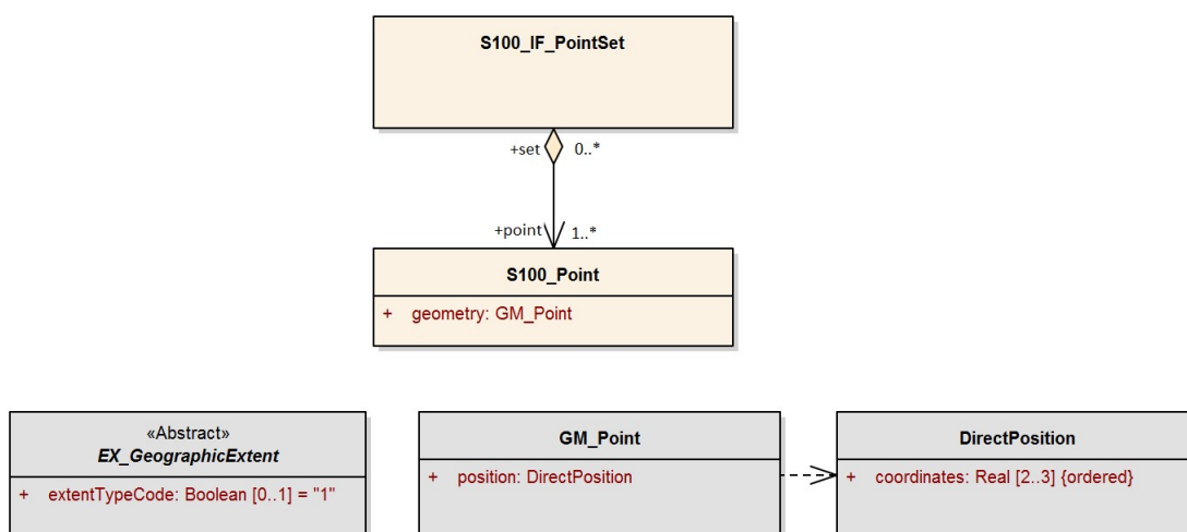
Figure 8-21 – S100_Point
