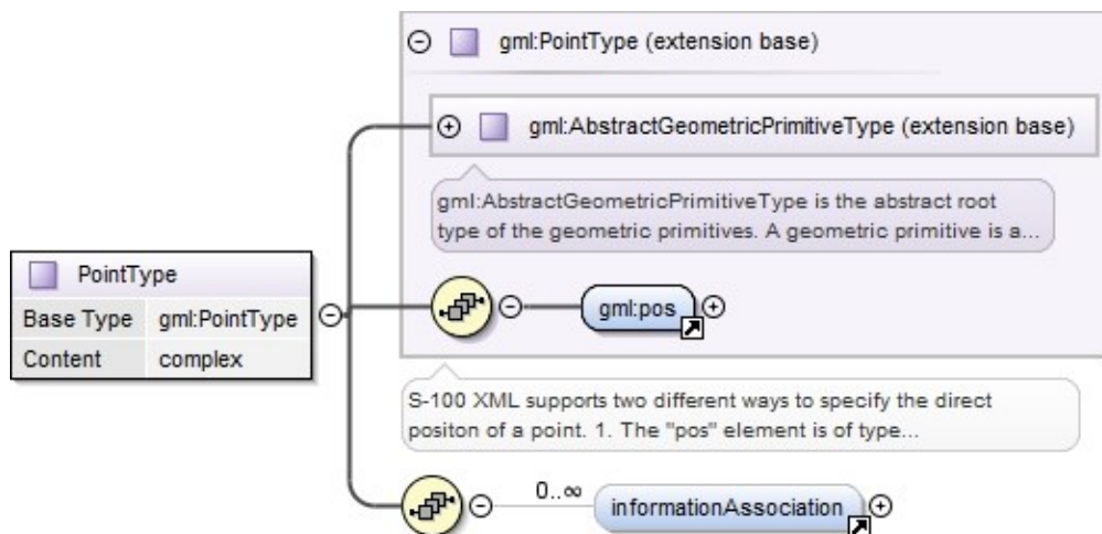
Figure 10b-9 – S-100 generic S-100 spatial type for point spatial object
