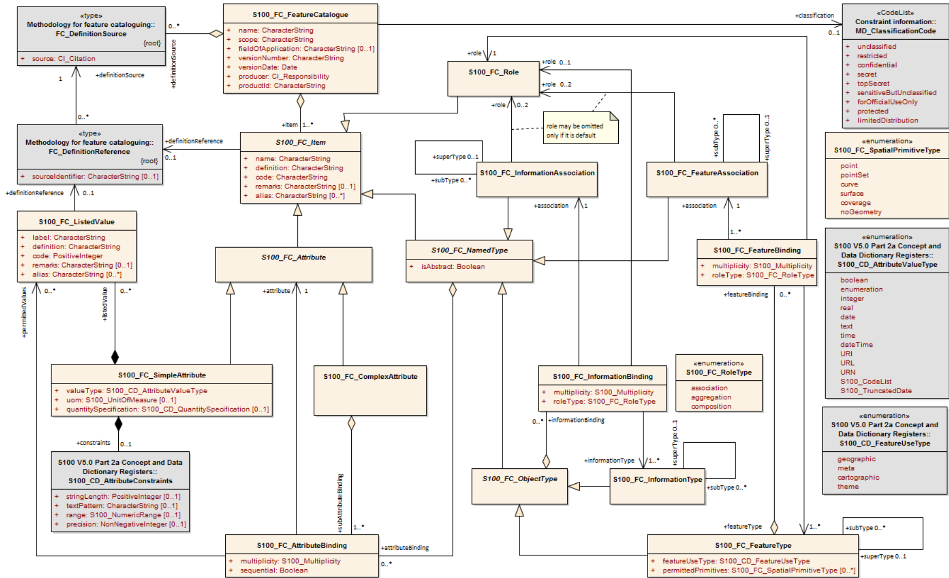
Figure 5-A-1. Feature Catalogue — UML Model
