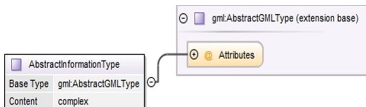
Figure 10b-7 – Base type definition for S-100 feature elements
