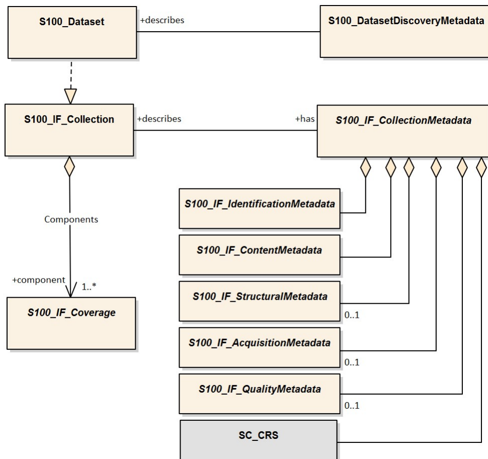
Figure 8-28 – Relationship to metadata
