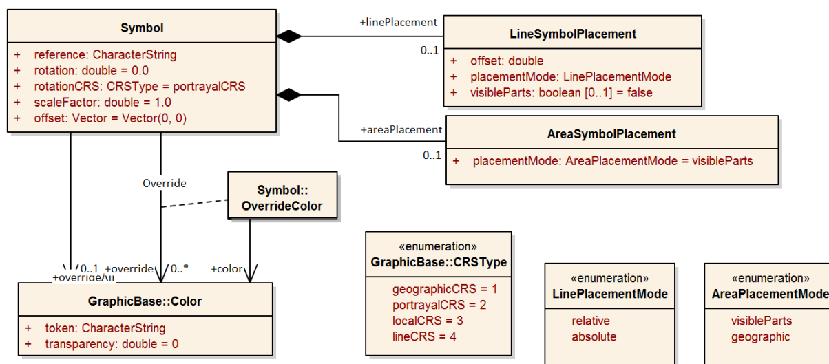
Figure 9-15 — Symbol Package
