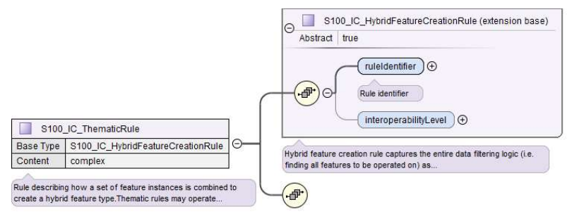
Figure 16-A-12 - Structure of S100_IC_ThematicRule
