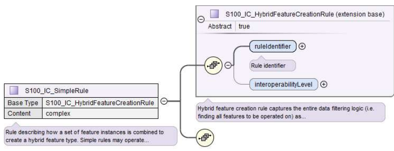
Figure 16-A-13 - Structure of S100_IC_SimpleRule
