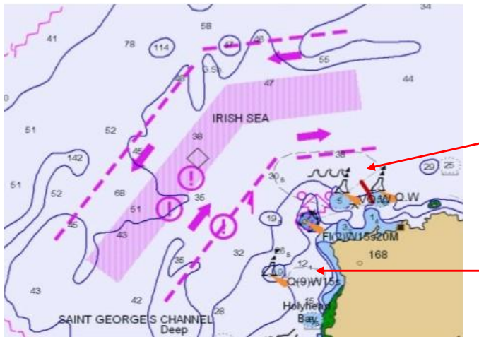
Figure 26– Traffic Separation Scheme with masked CTNARE
