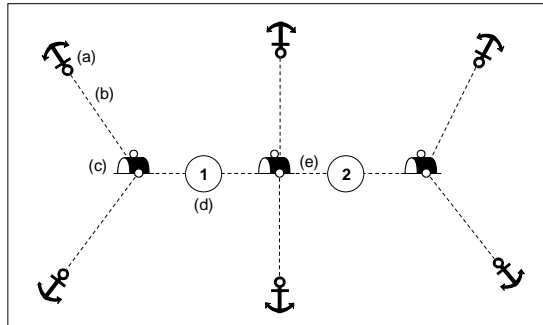
Figure 9 – Mooring trot
