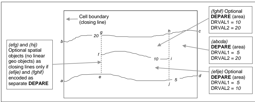
Figure 5 – Geometry of depth areas
