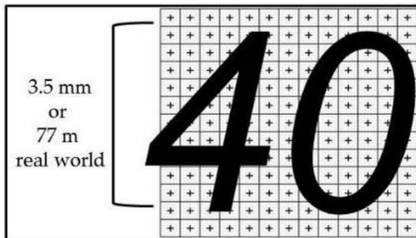
Figure H 3 - Charted Soundings vs. 6-metre S-102 Grid
