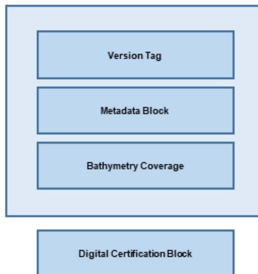
Figure 4-1 - Overview Structure of S-102
