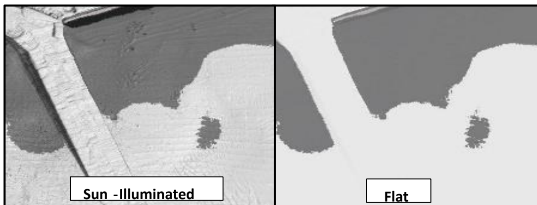
Figure 9-1 - Sun-illuminated and Static (Flat) Shading
