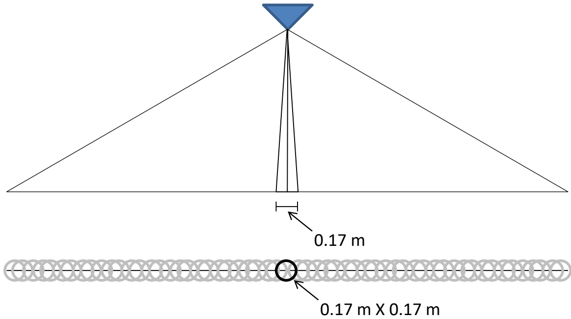
Figure H 1 – Sonar Footprint at Nadir
