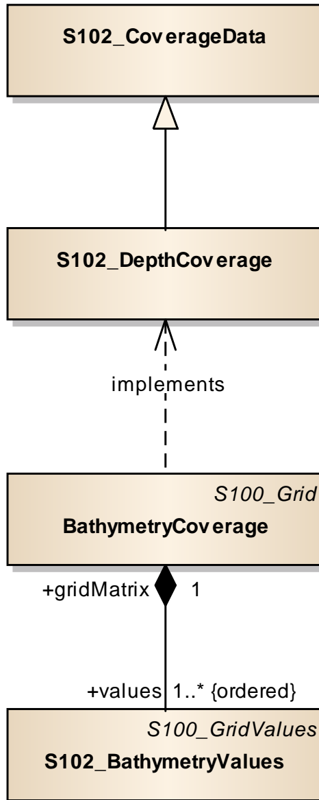
Figure 4-3 - Coverage Structure of S-102
