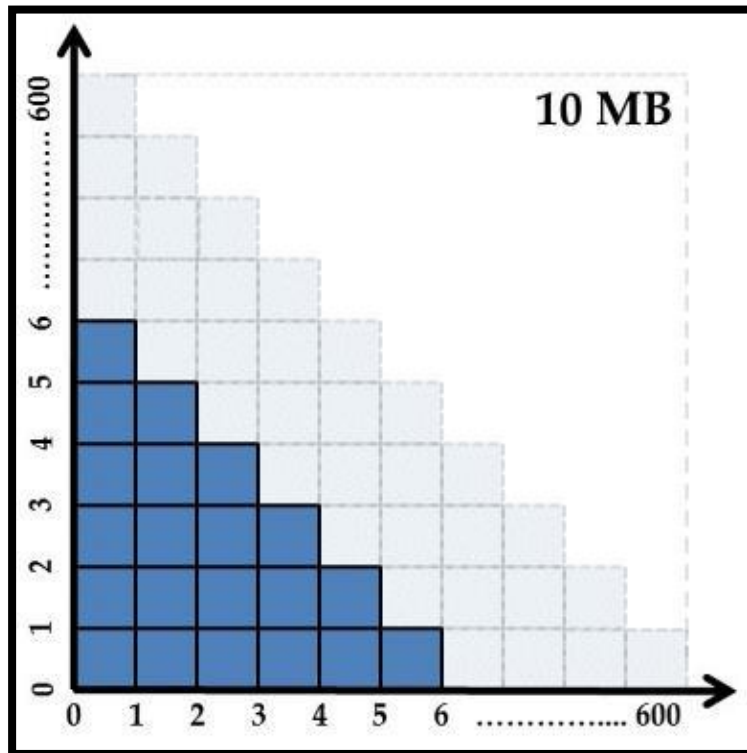
Figure E 1 - Informative grid extents for a 10 MB Uncompressed Dataset
