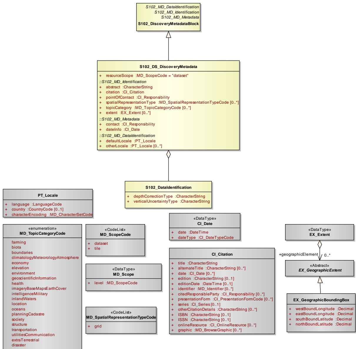
Figure 12-1 - S-102 Discovery Metadata
