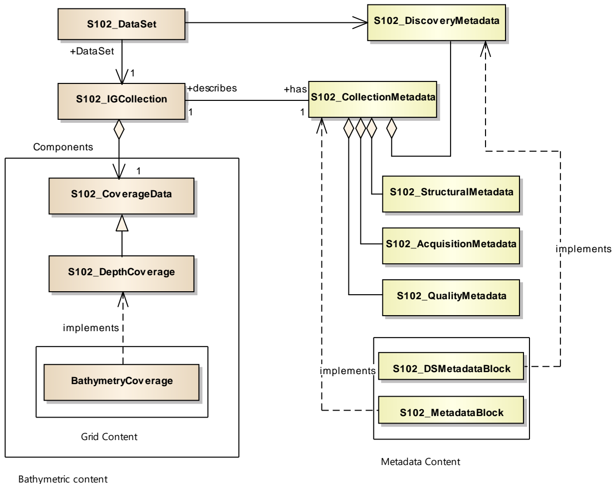
Figure 4-2 - Data Set Structure of S-102
