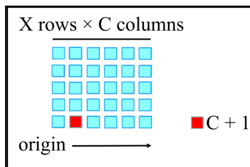
Figure 4-5 - S-102 Grid Node Location
