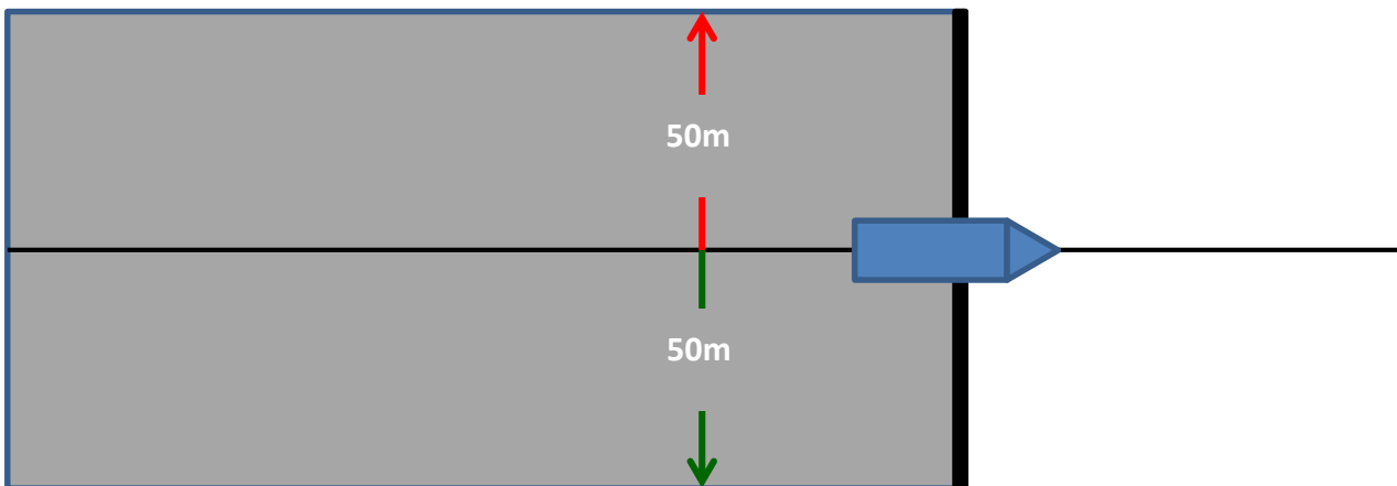
Figure H 2 - Swath Coverage of survey vessel
